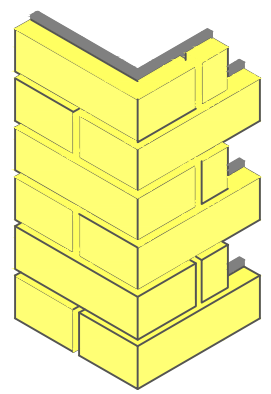
Right hand Flemish Reveal
